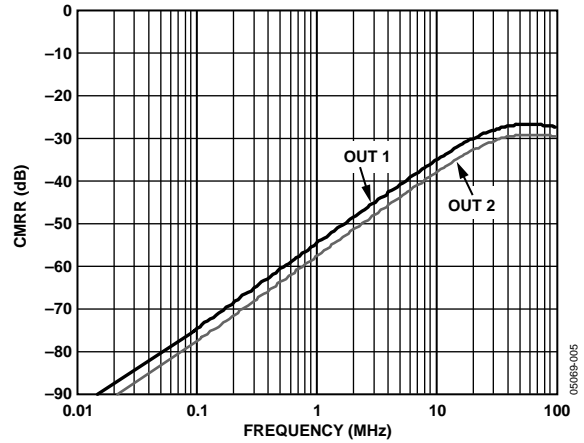
Figure 8. Common-Mode Rejection vs. Frequency ( V_S = \pm 5\text{ V} , R_L = 25\ \Omega )
