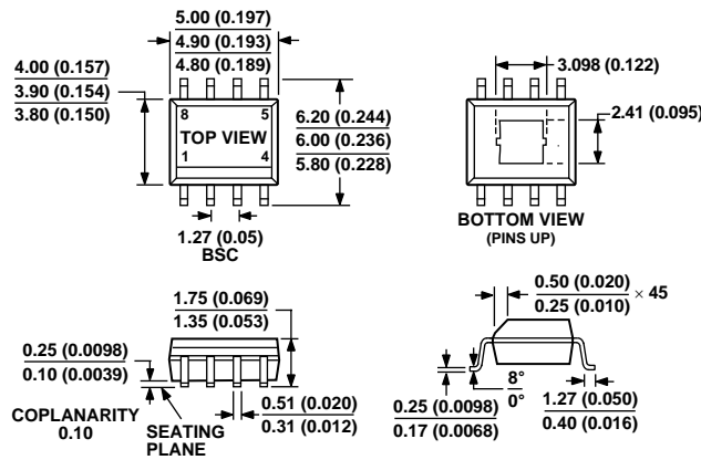
Figure 25. 8-Lead Standard Small Outline Package [SOIC] Narrow Body (R-8) Dimensions shown in millimeters and (inches)
